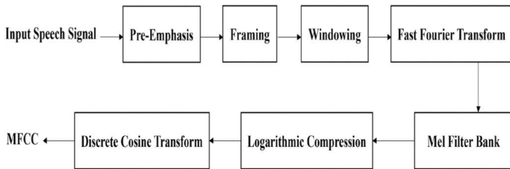
Gambar 2.2 Pipeline ekstraksi Mel-Frequency Cepstral Coefficients (MFCC)
