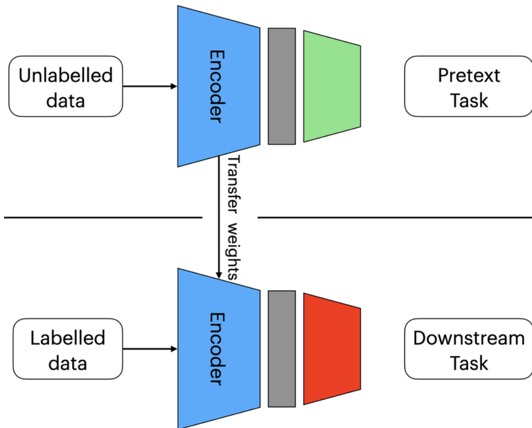
Gambar 2.4 Alur umum pembelajaran Self-Supervised
