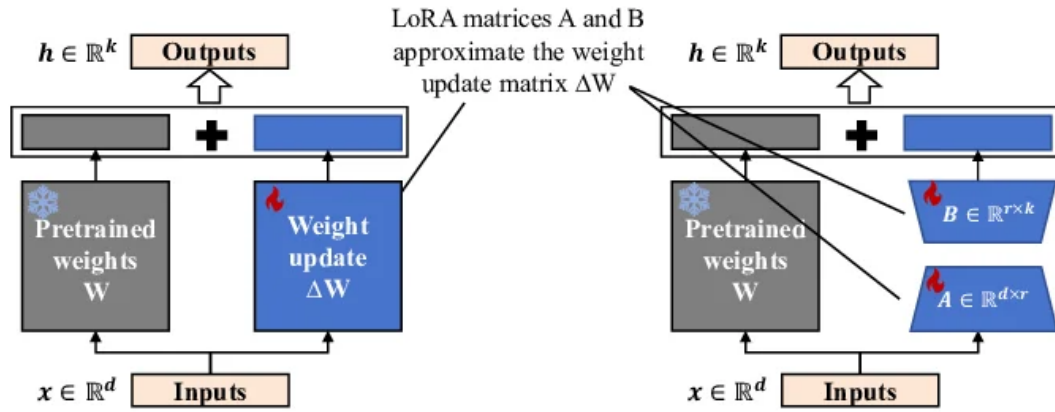
Gambar 2.6 Perbandingan full fine-tuning dan LoRA
